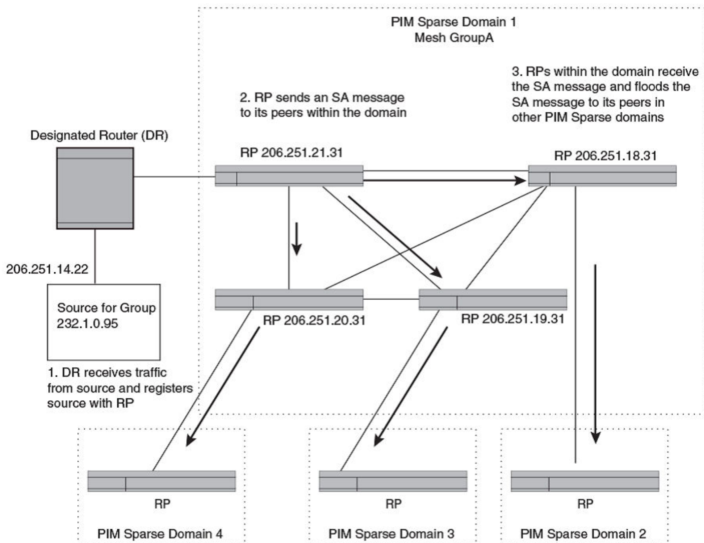
FIGURE 8 Example of MSDP mesh group
