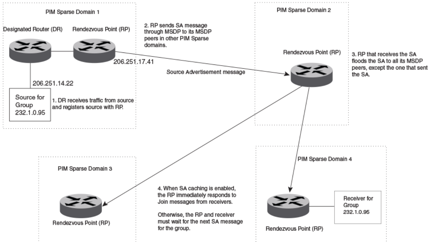
FIGURE 7 PIM Sparse domains joined by MSDP devices
